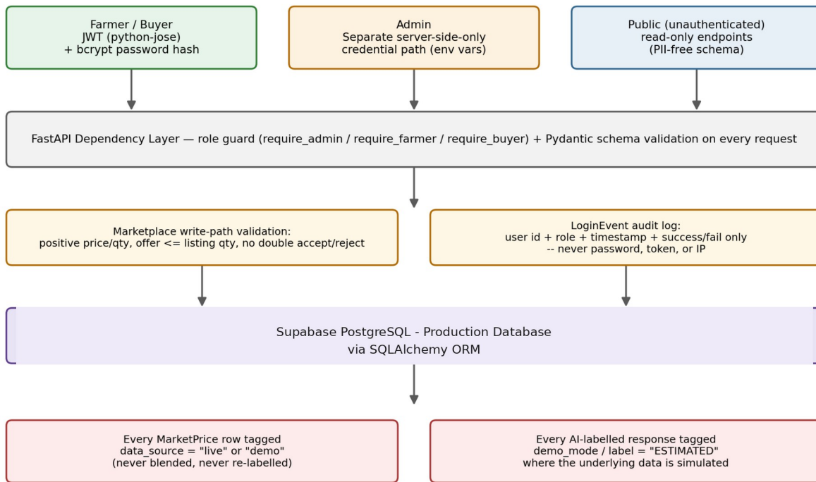
Figure 11. Security, Access Control, and Data-Provenance Architecture
